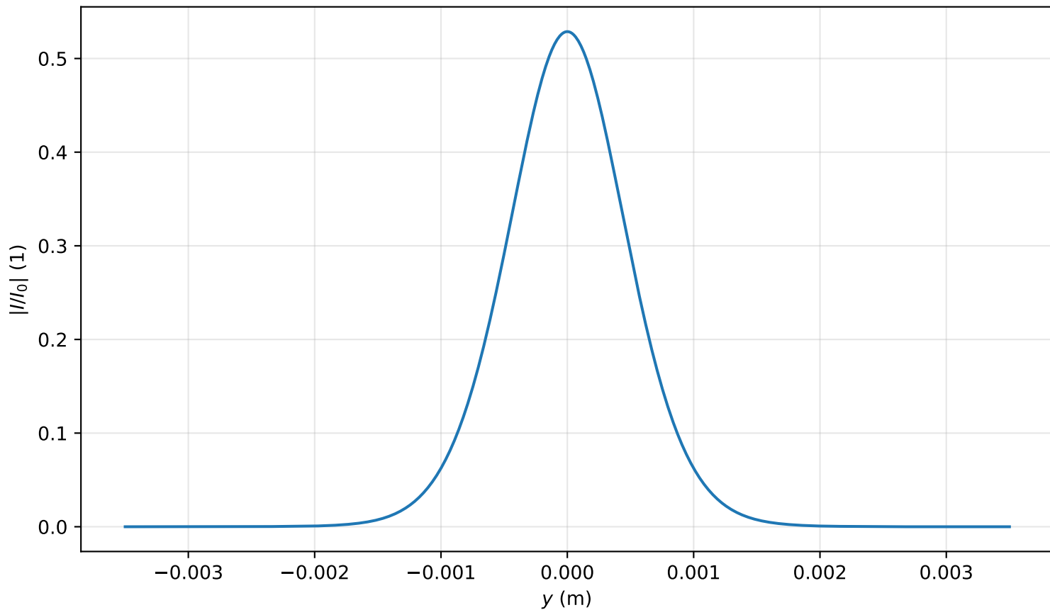
Intensity profile I(x=0, y, z=2.786)/I_0 , P_{in}=0.4P_{cr} , artificial time
